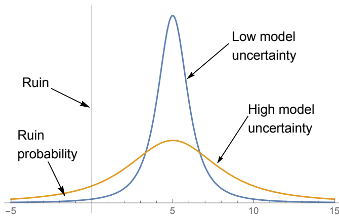
Figure 6: The more uncertain or skeptical one is of "scientific" models and projections, the higher the risk of ruin, which flies in the face of the argument of the style "skeptical of climate models". No matter how increased the probability of benefits, ruin as an absorbing barrier, i.e. causing extinction without further recovery, can more than cancel them out. This graph assumes changes in uncertainty without changes in benefits (a mean-preserving sensitivity) –the next one isolates the changes in benefits.
