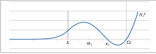
Figure 11: The Transfer function H for different portions of the distribution: its sign flips in the region slightly below \Omega
