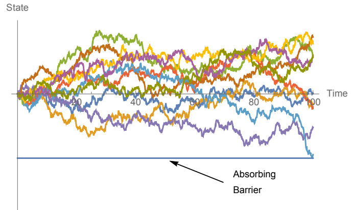
Figure 2: A variety of temporal states for a process subjected to an absorbing barrier. Once the absorbing barrier is hit, the process terminates, regardless of its future potential.
