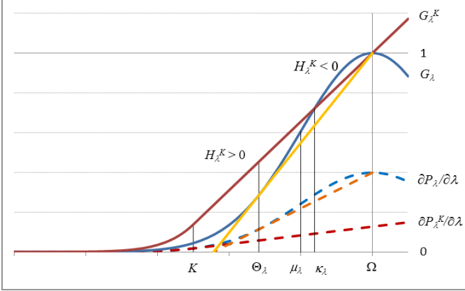
Figure 12: The distribution of G_\lambda and the various derivatives of the unconditional shortfalls
