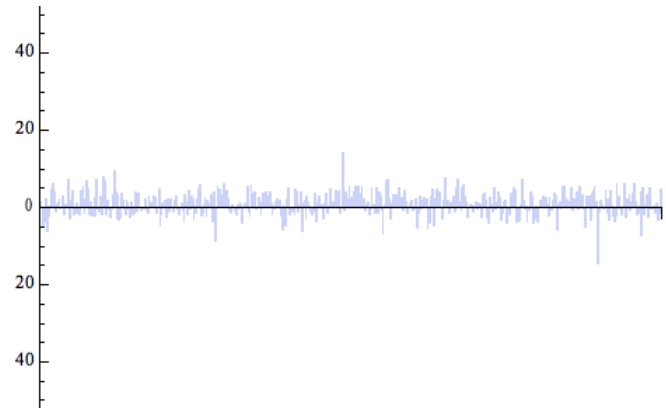
Figure 3: Thin Tails from Tinkering, Bottom-Up, Evolution. In nature no individual variation represents a large share of the sum of the variations. Natural boundaries prevent cascading effects from propagating globally. Mass extinctions arise from the rare cases where large impacts (meteorite hits and vulcanism) propagate across the globe through the atmosphere and oceans.
