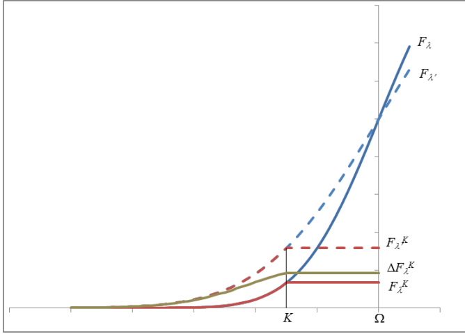
Figure 10: The different curves of F_\lambda(K) and F_{\lambda'}(K) showing the difference in sensitivity to changes at different levels of K .
