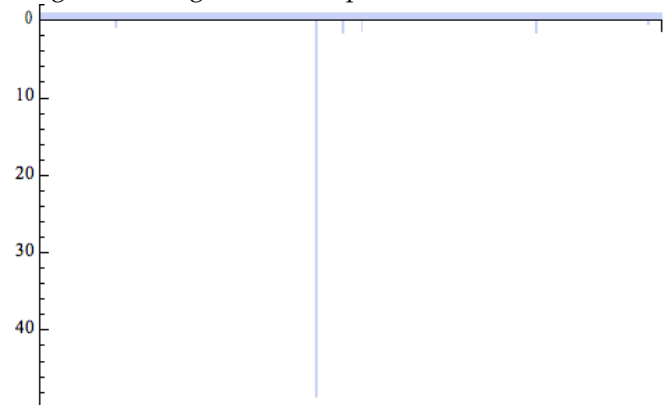
Figure 4: Fat Tails from a Top-Down, Engineered Design. In human made variations the tightly connected global system implies a single deviation will eventually dominate the sum of their effects. Examples include pandemics, invasive species, financial crises and monoculture.
