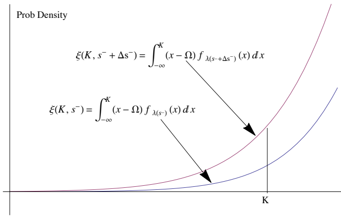
Figure 9: A definition of fragility as left tail-vega sensitivity, in other words how an increase in uncertainty (which includes errors) affects adverse outcomes . The figure shows the effect of the perturbation of a measure of the lower semi-deviation s^- on the tail integral \xi of (x - \Omega) below K , \Omega being a centering constant. Centrally, our detection of fragility does not require the specification of f the probability distribution.
