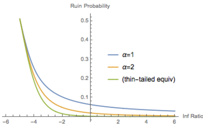
Figure 7: The graph shows the asymmetry between benefits and harm and the effect on the ruin probabilities. Shows the effect on ruin probability of changes the Information Ratio, that is, \frac{\text{expected benefit}}{\text{uncertainty}} (or signal divided by noise). Benefits are small compared to negative effects. Three cases are considered, two from Extremistan: extremely fat-tailed ( \alpha = 1 ), and less fat-tailed ( \alpha = 2 ), and one from Mediocristan.
