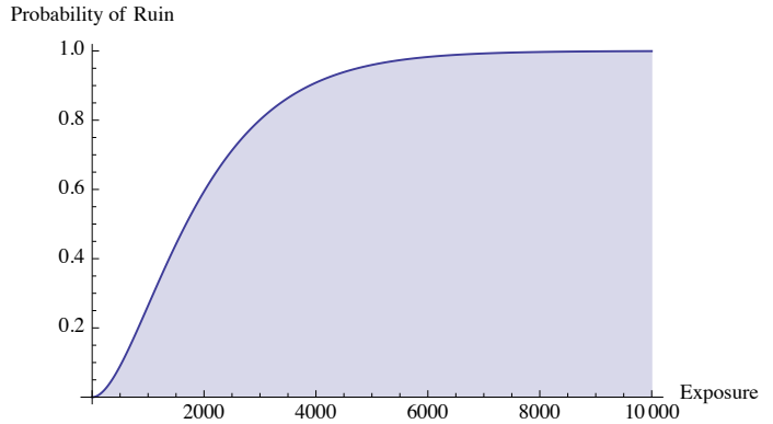
Figure 1: Why Ruin is not a Renewable Resource. No matter how small the probability, in time, something bound to hit the ruin barrier is about guaranteed to hit it.
