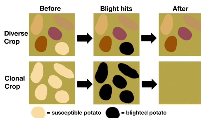
Figure 8: A simplified illustration of the mechanism behind the potato famine of the 19 th C. showing how concentration from monoculture increases the risk of ruin. Inspired by Berkeley’s Understanding Evolution .
